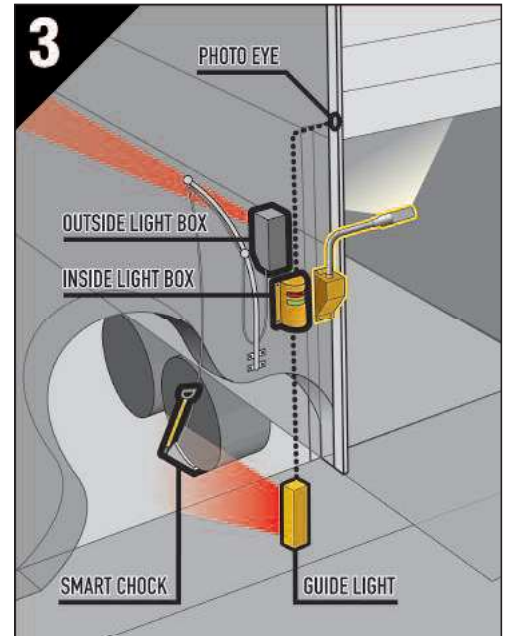
3 Add on with DL Manufacturing Smart Chock™ or Safety Signal™ – Guide Light mirrors red and green signal lights of the outside communication box
